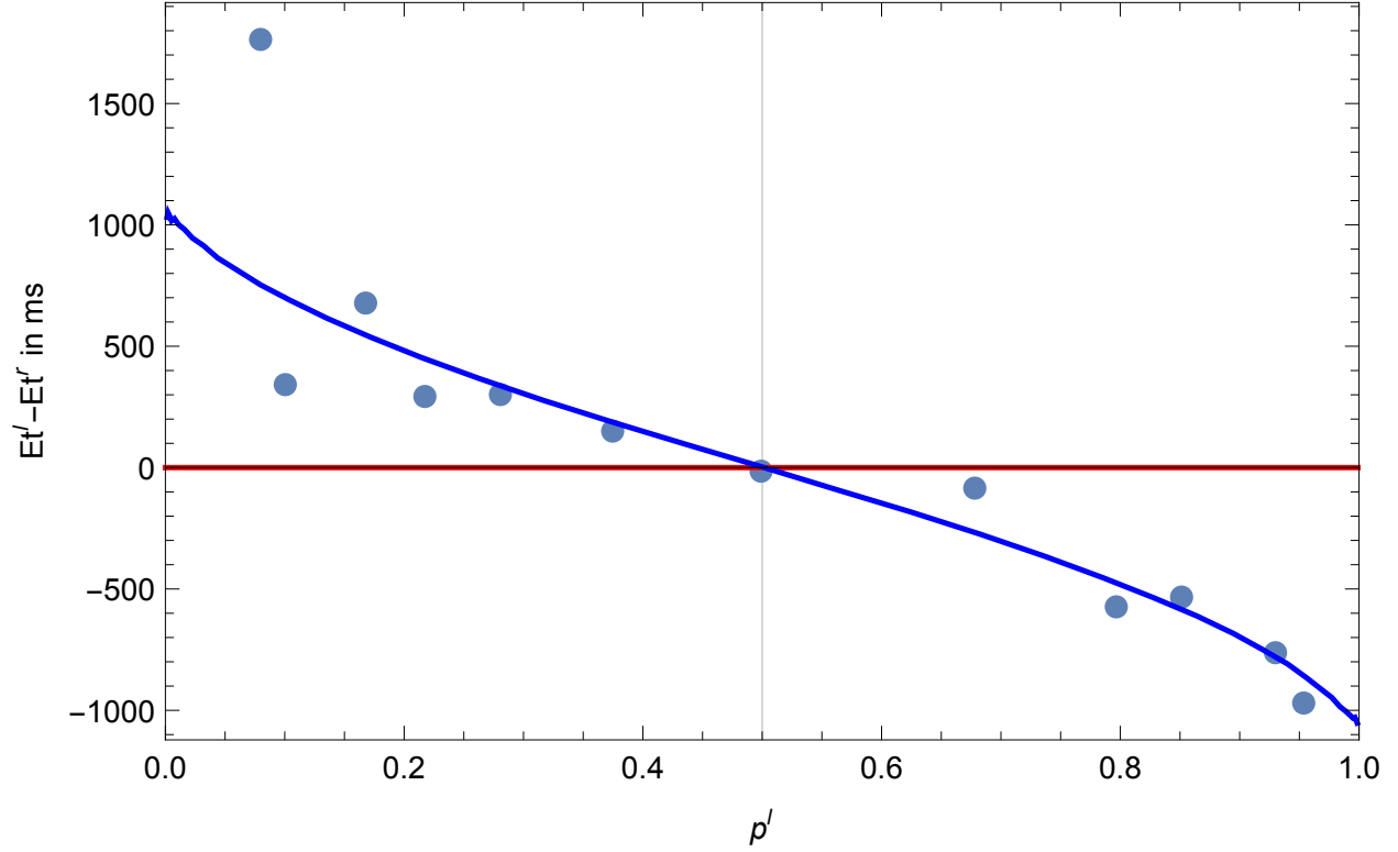
Figure 1: The dots display the data from an experiment by Krajovich, Armel, and Rangel (2010) . Since each alternative pair is sampled only once, we used self-reported rankings to cluster pairs by self-reported item rankings. The blue line displays simulations of the approximately optimal barrier \bar{b} for the uncertain-difference DDM (derived in Section 3.3) with parameters c = 0.05, \sigma_0 = \alpha = 1 ; each simulation uses 5 \cdot 10^6 draws and time is discretized with dt = 0.01 . The expected time to choose l is lower than the expected time to choose r for pairs of alternatives where l is the modal choice; it is higher for pairs where r is modal. The red line displays predictions of the simple DDM for any combination of parameter values.
